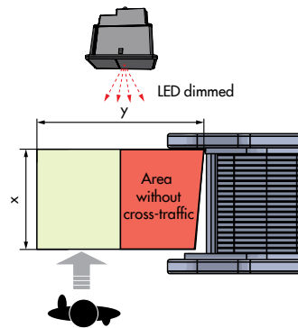
Figure 12: Detection field free; Person moves to cross the escalator entrance area. LED status is dimmed.
