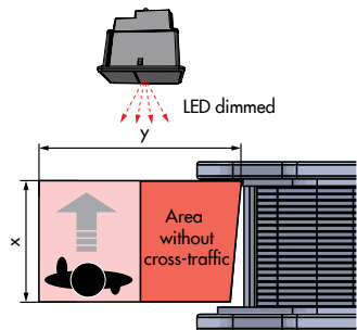
Figure 13: Sensor recognizes the person is moving cross the escalator entrance. LED status remains dimmed → no output switched.
