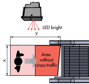
Figure 11: Person is detected entering detection area, moving towards the escalator entrance area. LED status is bright.
