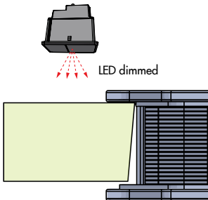
Figure 16: The detection field is free.
